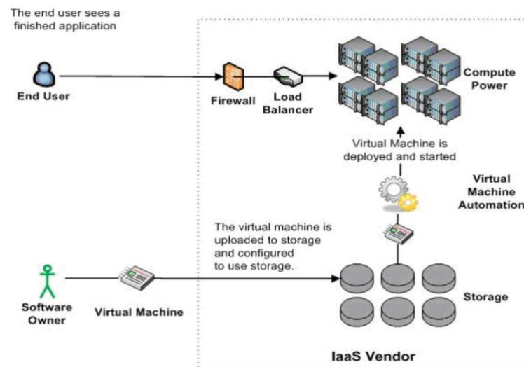
Slika 3 Infrastructure as a service, Izvor: Sushil Bhardwaj, Leena Jain, Sandeep Jain; Cloud computing: A study of infrastructure as a service (IAAS) , « International Journal of Engineering and Information Technology », sv. 2, br. 1, pp. 60-63, 2010.
