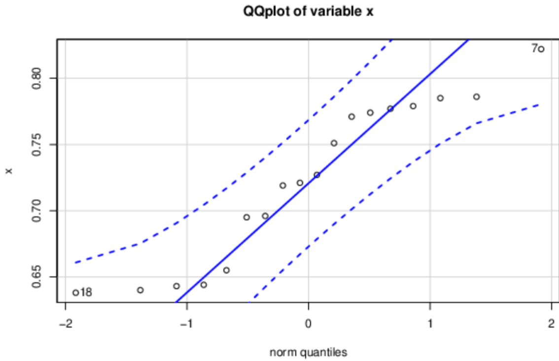
Chart 79: Output PEARSON correlation, QQ-plots, Poland
