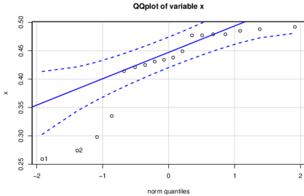
Chart 55: Output PEARSON correlation, QQ-plots
