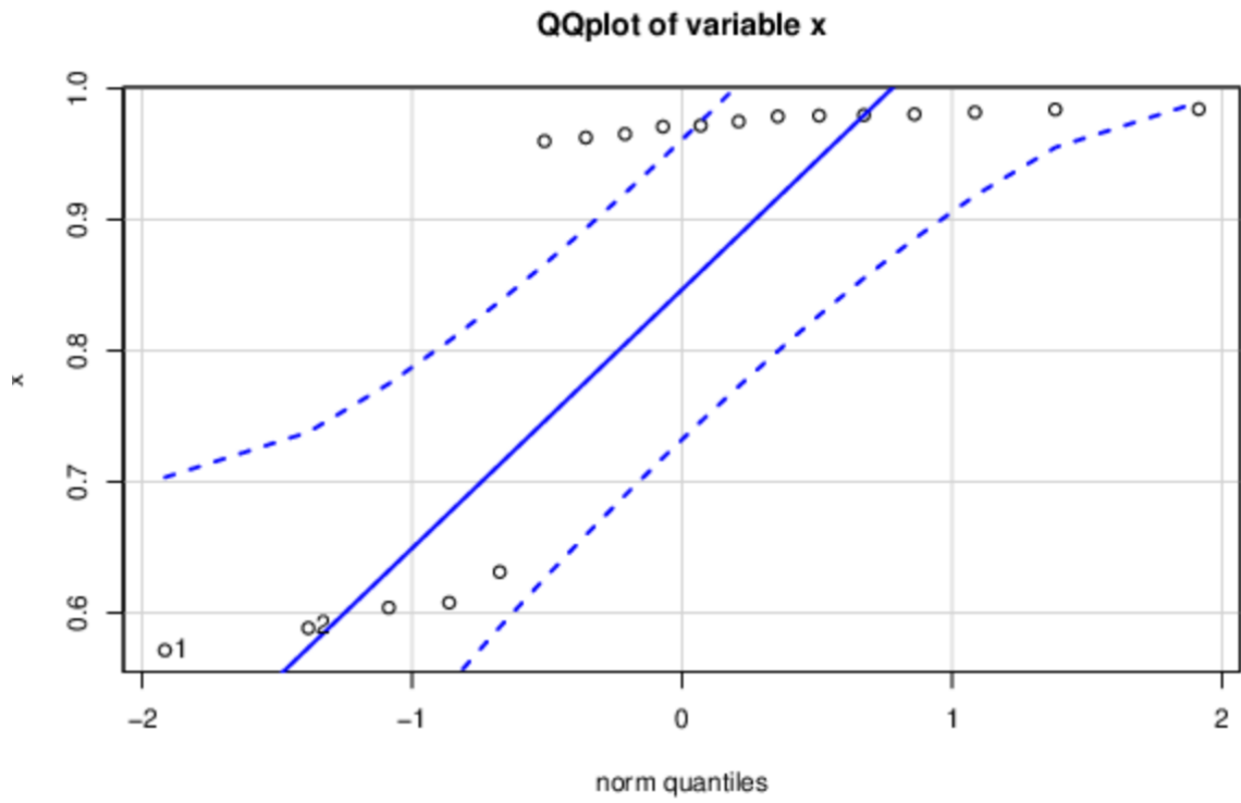
Chart 75: Output PEARSON correlation, QQ-plots, Czech Republic
